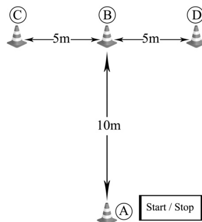
FIG. 1. Diagram of T-test.
