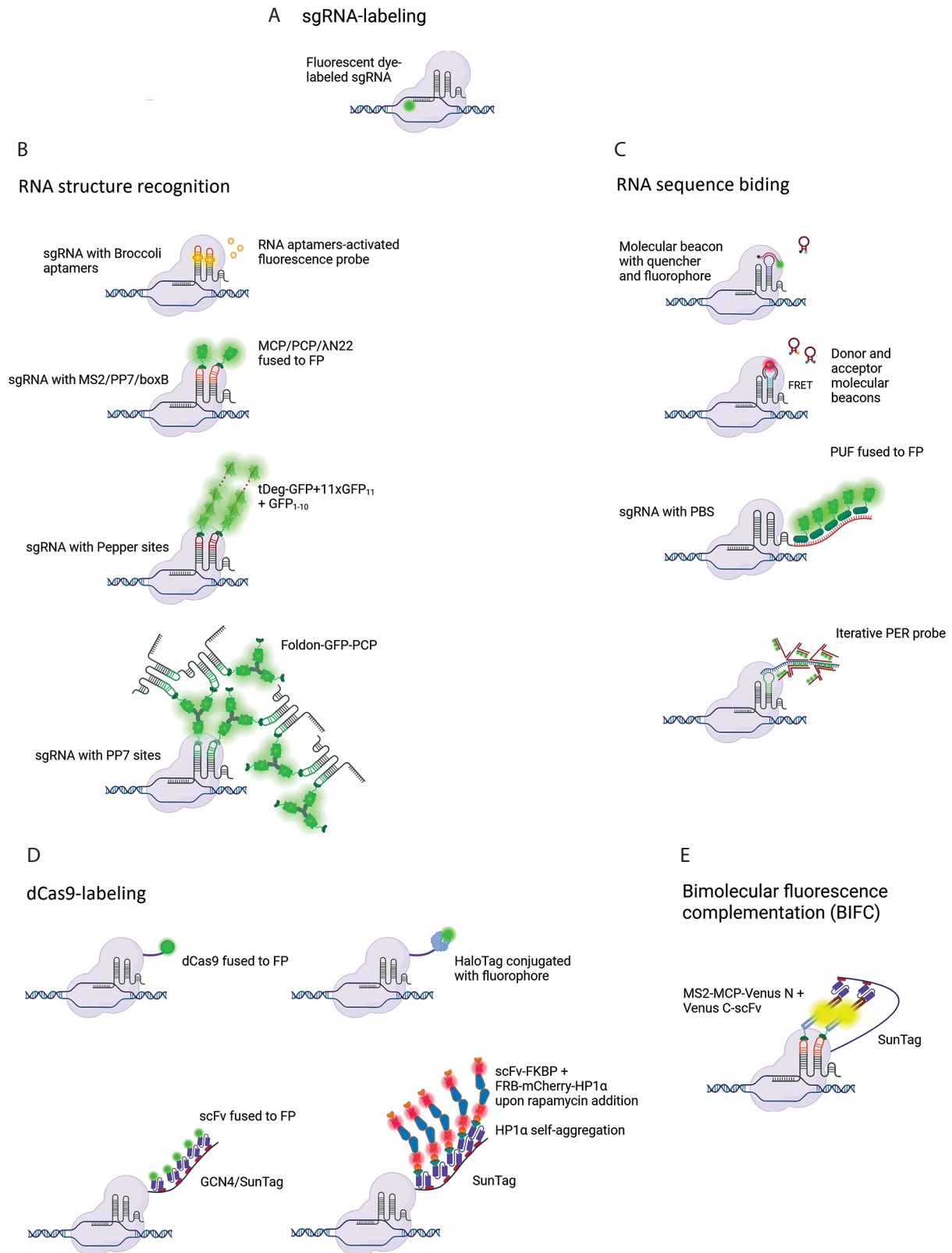
Figure 1. Development of CRISPR-based imaging systems. sgRNA-labeling methods include (A) direct labeling of the sgRNA with a fluorophore, (B) methods relying on RNA sequence recognition, and (C) methods based on the recognition of structural motifs incorporated into the sgRNA. (D) Methods based on dCas9 labeling. (E) A combined approach based on bimolecular fluorescence complementation. Created in BioRender
